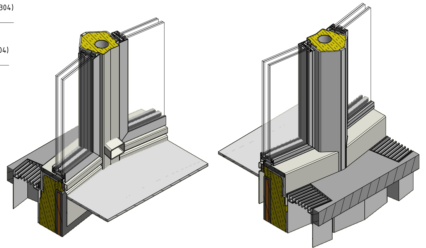
ISOMETRIC VIEW FROM OUTSIDE
