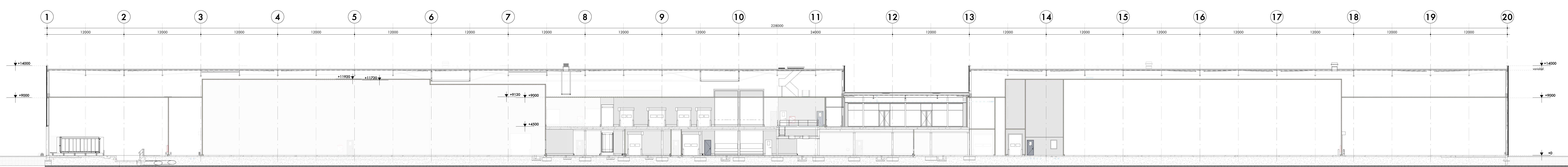
Doorsnede tussen as J-K 1:200
