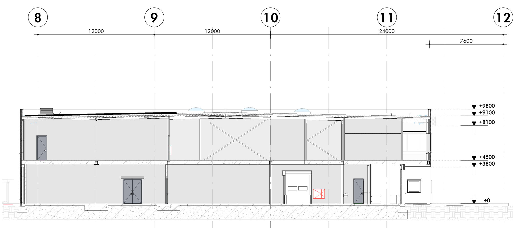
Doorsnede tussen as K-L
