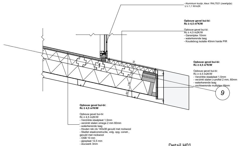
Detail H01
