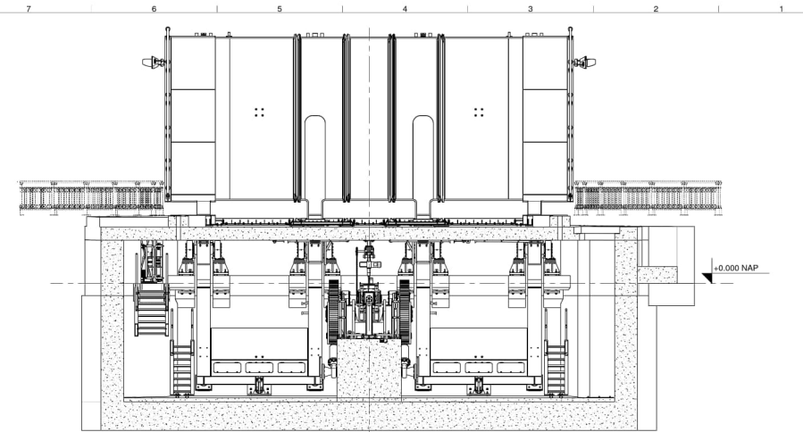
L-L (1:50)
