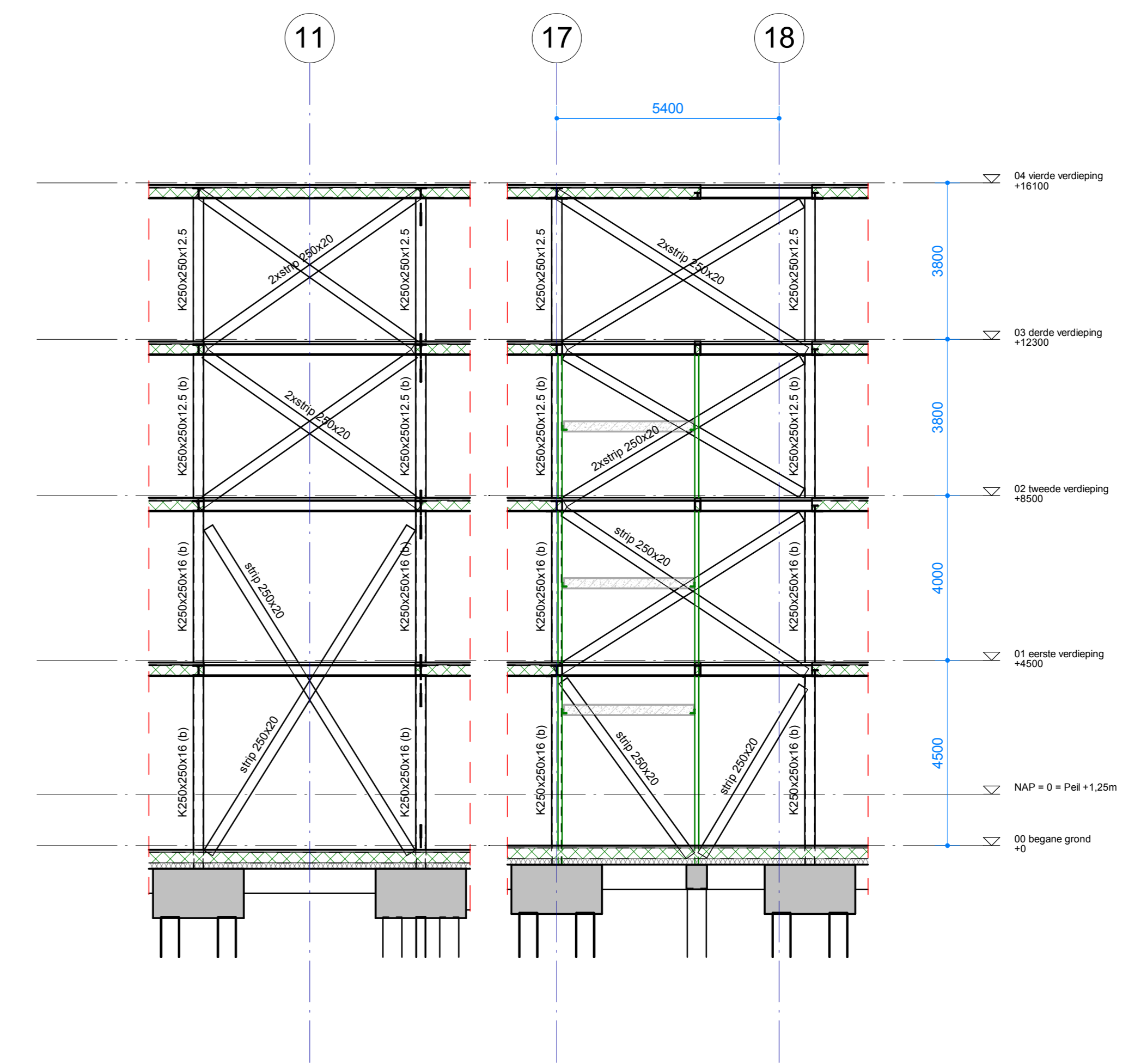
Doorsnede C (as F)
