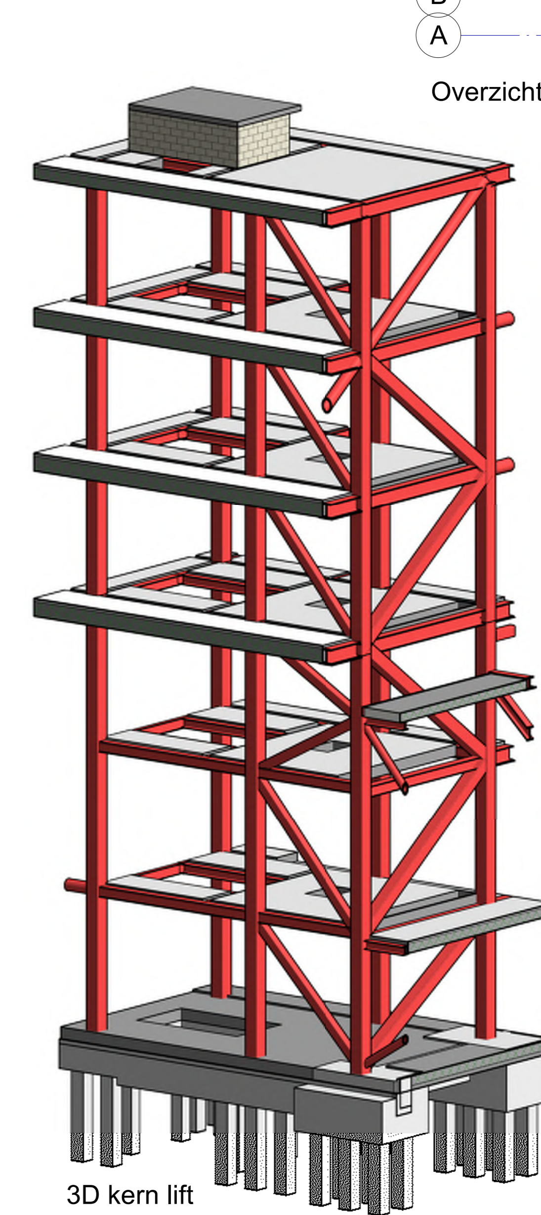
3D kern lift
